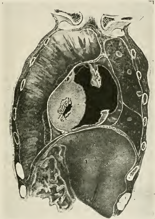
FIG. 345.—Massive left-sided empyema occupying practically the whole pleural cavity. The lung is represented by two small fibrous masses adherent to the pericardium which contains a small serous effusion. The heart, which is enlarged, is filled with blood clot. The diaphragm is pushed downward and the right lung greatly compressed. ( Pirogoff. )
